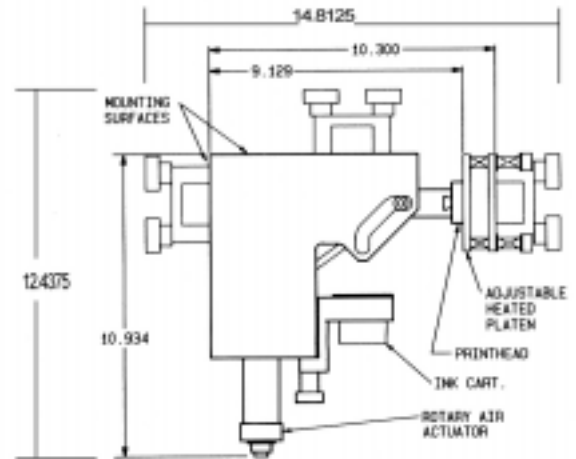
US5000 Dimensional Drawing
